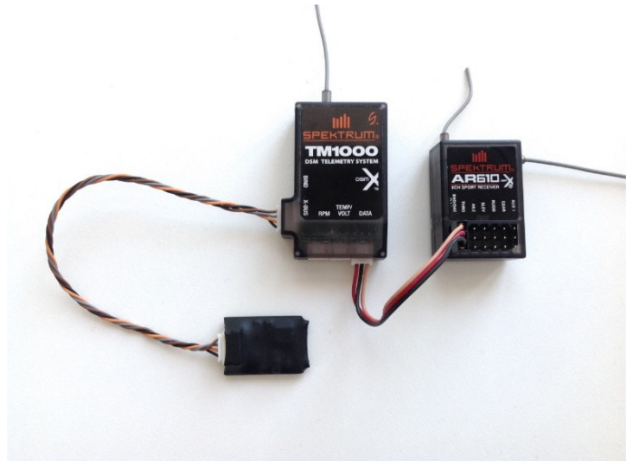
Figure 2: Connection Scheme Alti-DX2 - TM1000 - Receiver
